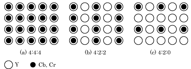
Fig. 1 Illustrations of YCbCr color formats.
