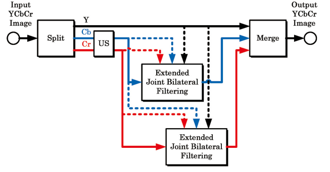
Fig. 4 Block diagram of the filtering process for chroma images based on extended joint bilateral filtering.
