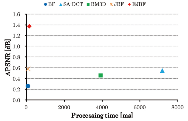
Fig. 15 Graph of \Delta PSNR vs. processing time for each method.
