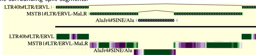
Figure 4 Example of nested insertions. This region of the human genome (hg38, chr11:11990878..11991874) exemplifies nested transposable element insertions. Here, an instance of AluJr was inserted within an instance of MSTB1, which itself was inserted into an instance of LTR40b. The confidence heatmap is included for reference, and demonstrates a change-point decision in the context of nested annotations; heatmaps for competing annotations are not shown, in order to reduce visual clutter. PolyA automates the splicing of inserted elements and stitching of the surrounding split segments.
