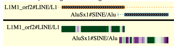
Figure 2 Detecting the change-point between overlapping elements; demonstration of confidence heatmap. This region of the human genome (hg38, chr10:58800-59500) contains a fragment of an L1M1 element, overlapping the tail of an AluSx1 candidate annotation. The heatmap on the bottom represents the position-specific confidence computed in PolyA, with dark green = high confidence, dark purple = low confidence, and moderate confidence represented by lighter colors and white. To limit visual clutter, this heatmap shows only the confidence heatmaps for the two 'winning' annotations; others are hidden from view. The top half of the figure shows the final PolyA adjudication, in which the region in which the competing annotations overlap is assigned to the higher-confidence L1M1 annotation.
