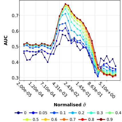
Figure 3: Max- k effect for COMPASS-R on Flickr.
