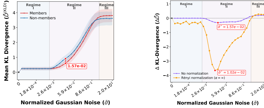
Figure 1: Perturbation sensitivity and membership divergence across normalized Gaussian noise on a Flickr pre-training target set against LLaVA v1.5–7B model with k=0.9 . Left: Mean unnormalized KL divergence for members and non-members, with shaded bands denoting one standard deviation. Their similar response in Regime I produces a near-zero divergence gap, whereas members exhibit greater divergence in Regime III. Right: The member–non-member gap \Delta\bar{D} = \bar{D}_m - \bar{D}_n with and without Rényi normalization ( \alpha = \infty ). Rényi normalization amplifies the negative gap in Regime II. Red markers indicate the noise level minimizing \Delta\bar{D} for each metric.
