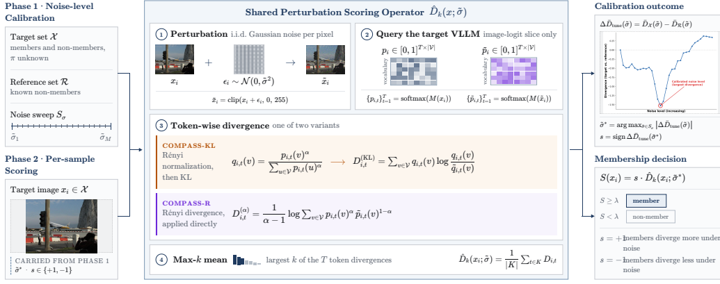
Figure 2: COMPASS attack structure. In the tuning phase, COMPASS compares the divergence responses of the unlabeled target set and a known non-member reference set across candidate noise levels to select the perturbation magnitude and score direction. In the scoring phase, it applies the selected perturbation to each target image, aggregates the largest token-wise divergences, and orients the result to produce a membership score.
