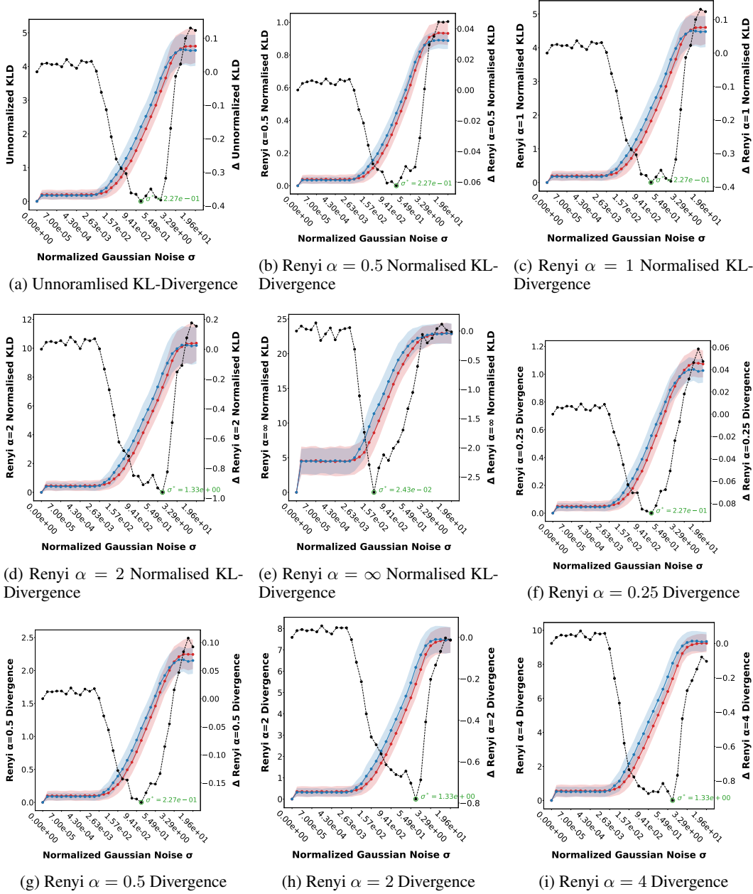
Figure 7: Raw divergence curves for all tested normalization for a flickr target subset members (red), non-members (blue), and member-non-member difference (black) against the MiniGPT-4o model.
