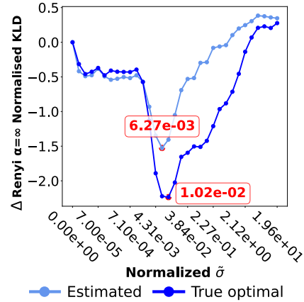
Figure 4: Effectiveness of noise-level tuning. Top: AUC using the true optimal noise level and the noise level estimated by our tuning procedure. Right: Estimated and true optimal noise levels for Rényi- \infty normalized KL divergence difference. The estimated \tilde{\sigma} lies near the true optimum and yields performance close to the ideal setting.
