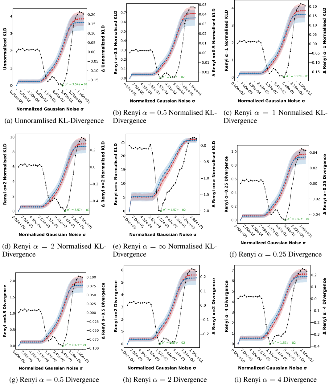
Figure 6: Raw divergence curves for all tested normalization for a flickr target subset members (red), non-members (blue), and member-non-member difference (black) against the LLaVA model.
