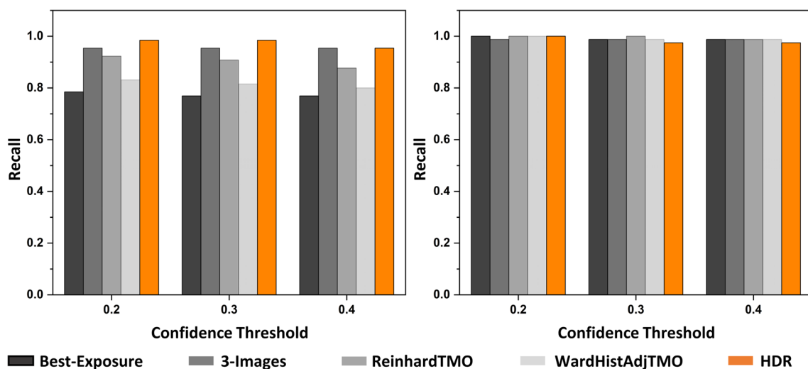
Fig. 8 Column plots for recall of (a) defect group green and (b) defect group blue
