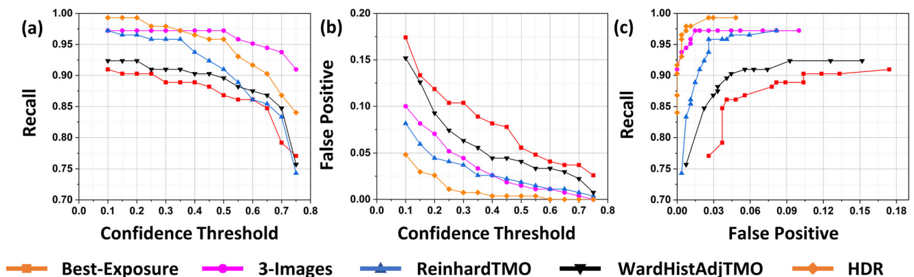
Fig. 4 (a, b) Recall and false positive plots respectively with respect to confidence threshold, and (c) receiver operating characteristic (ROC) curve at IOU threshold of 0.5
