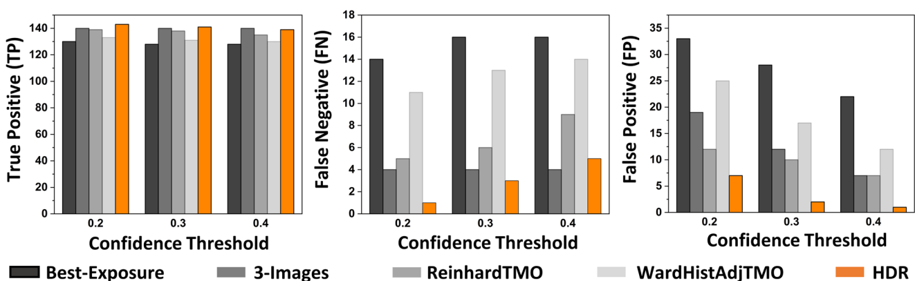
Fig. 5 Column plots of (a) true positives, (b) false negatives and (c) false positives at confidence thresholds 0.2, 0.3 and 0.4 with IOU 0.5
