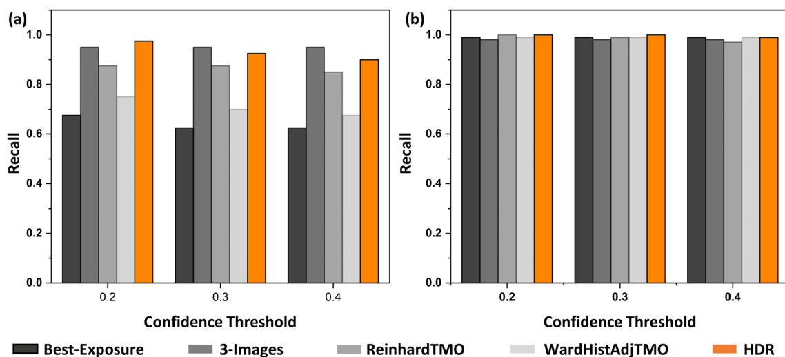
Fig. 9 Column plots for recall of (a) necks and (b) splits
