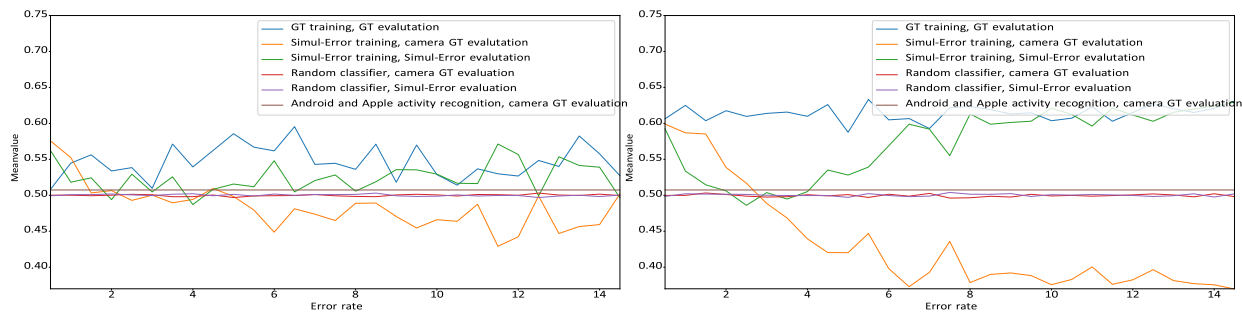
Figure 3: Random Forest, BIBO classification, AUC performance, left using BLE RSSI, right GPS (p-value with respect to random classifier on 0.5 value < 0.01)
