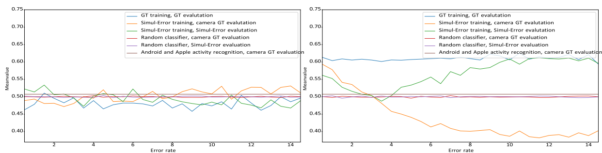
Figure 4: Multi Layer Perceptron, BIBO classification, AUC Performance, left using BLE RSSI, right using GPS (p-value with respect to random classifier on 0.5 value < 0.01)
