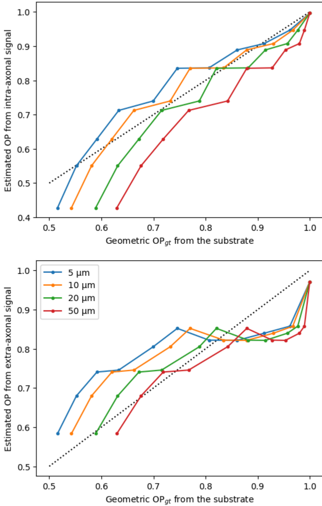
Figure 4: Estimated OP from the signal for our collection of substrates as a function of geometric OP gt computed from the substrate for several lengths of segments for the intra-cellular signal (top) and extra-cellular signal (bottom).
