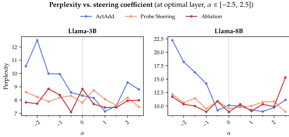
Figure 7. Perplexity of steered responses at the optimal layer.
