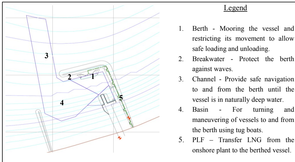
Figure 1. LNG terminal with berth 1150m offshore
