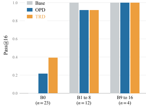
Figure 7: AMOBench Pass@16 by base-model difficulty for Qwen3-8B under OPD, with K=16 completions per question. The buckets contain questions with 0, 1 to 8, or 9 to 16 correct base-model completions, respectively. B0 contains the 23 questions left unsolved by the base model in all 16 attempts. OPD denotes the vanilla forward-KL baseline.
