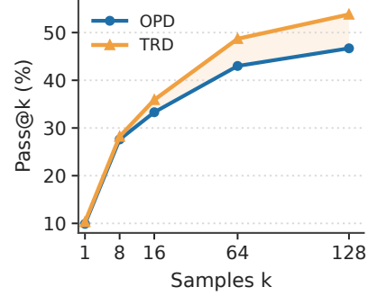
Figure 3: Pass@ k on AMOBench for Qwen3-4B-Instruct-2507 under the separate-teacher regime.
