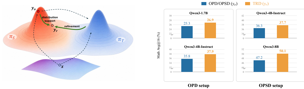
Figure 1: Left: TRD refines student-generated trajectories y_o into improved trajectories y_r , which are then used for distillation. Right: Mean Avg@16 across the five math benchmarks for OPD/OPSD and TRD under different base models.
