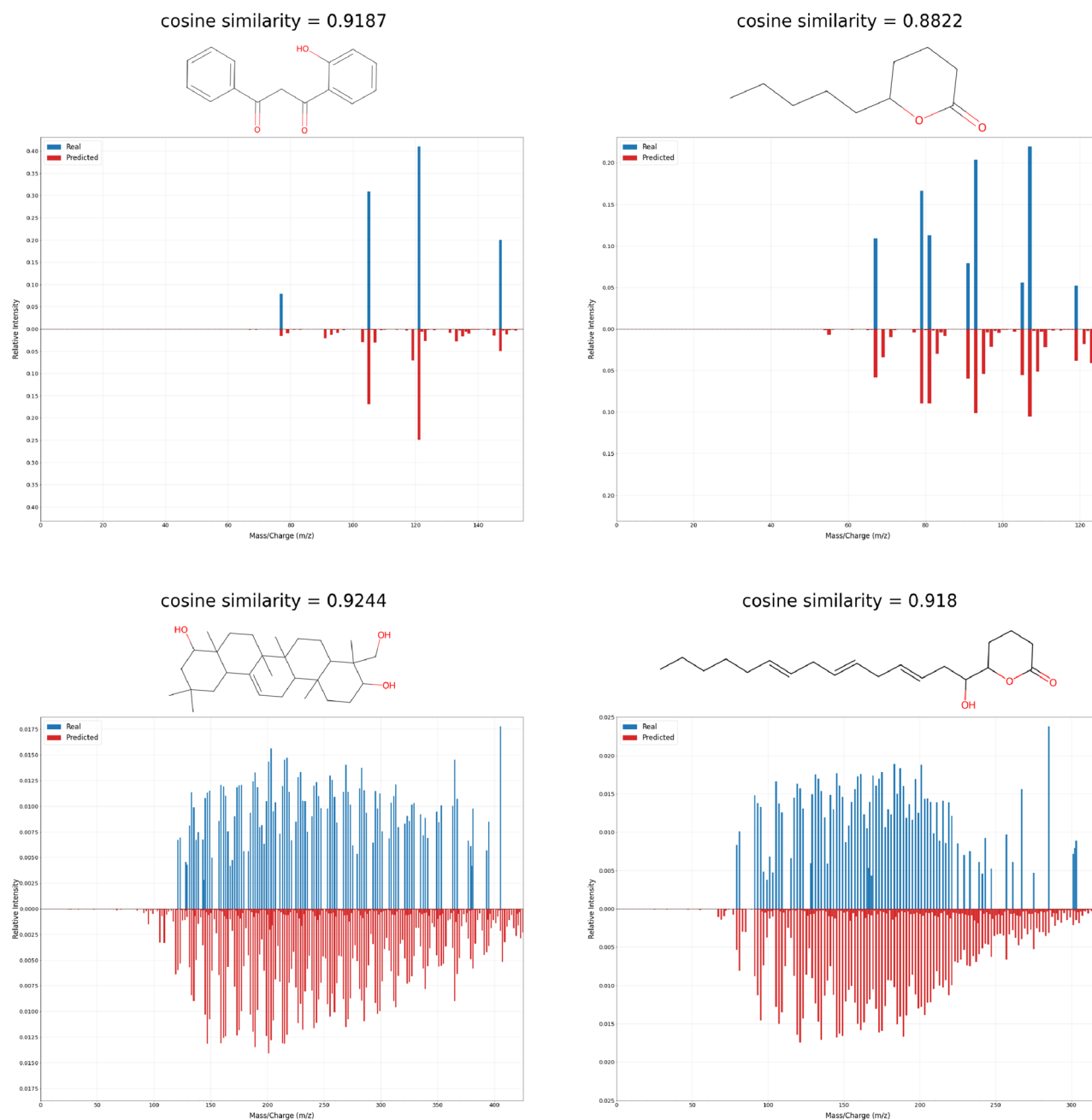
Figure 3. Examples of the real and predicted spectra for the four molecules. The real and predicted spectra exhibit comparable patterns, showcasing similar characteristics for complex molecular structures, irrespective of whether they contain an aromatic ring or not. However, it is noticeable that the predicted spectra display lower intensity, likely due to the presence of smaller peaks.
