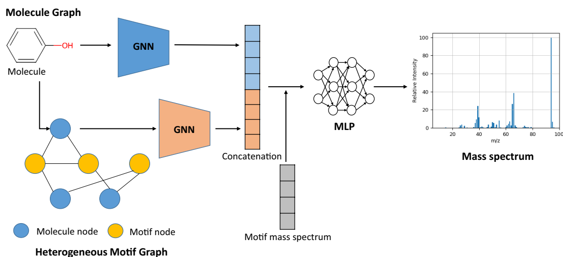
Figure 1. Overall architecture of MoMS-Net. The model consists of two GNN-based encoders, one for molecule graph and the other for heterogeneous motif graphs, respectively. Both types of graph embeddings from each GNN encoder are concatenated to form a single vector, and an MLP layer is finally applied to obtain the mass spectra prediction.
