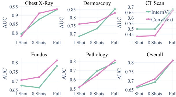
Figure 6. Few-shot performance on out-of-distribution datasets. InternVL represents the ViT-based model, while ConyNext represents the convolution-based model. In general, ViT-based models and ConyNext-based models exhibit similar overall performances across all shots, with ViT excelling at CT Scan tasks while ConyNext performs better at diagnosing fundus images.
