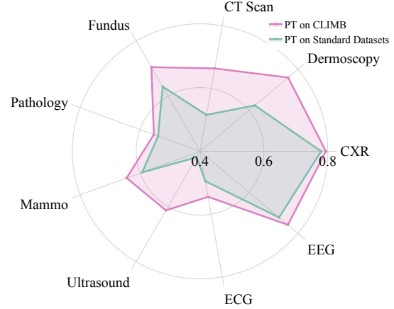
Figure 7. Few-shot performance of models across different pre-training (PT) datasets. CXR: Chest X-ray. We use ConvNextv2 for vision, ECG JEPA for ECG data, and BIOT for EEGs. PT on Standard Datasets is the performance of training one shot example on top of their own pretrained weights, while PT on CLIMB is the performance of training one shot example on top of our CLIMB dataset. For EEGs, 8 shot results are used instead due to the inherent complexity of the task.
