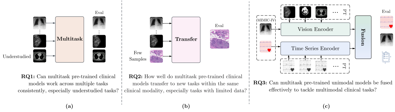
Figure 3. Experimental setup for evaluating (a) multitask, (b) transfer, and (c) fusion learning strategies, addressing RQ1, 2, 3 respectively. We show inputs to the model on the left and display evaluation on the right. (a) trains a single model on multiple clinical tasks across different medical modalities and evaluate on each individual dataset to see if model can generate across diverse tasks, including understudied ones. We compare the model’s performance across different architectures, as well as between the performance of single task learning versus multitask learning. (b) explores how well multitask pretrained clinical models transfer to new tasks, despite having few samples in the same modality. In this experiment, each model is trained on a few samples of a target out-of-distribution (OOD) dataset, as well as other tasks across different clinical modalities. (c) experiments on whether multitask pretrained unimodal models can be fused effectively to tackle multimodal clinical tasks. The source encoders are first separately trained with diverse data in their on modality, before being fused and evaluated on a new multimodal dataset (MIMIC-IV).
