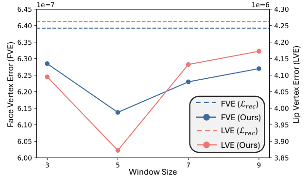
Figure 4: Performance analysis according to different window sizes of the viseme coarticulation weight in FVE and LVE.
