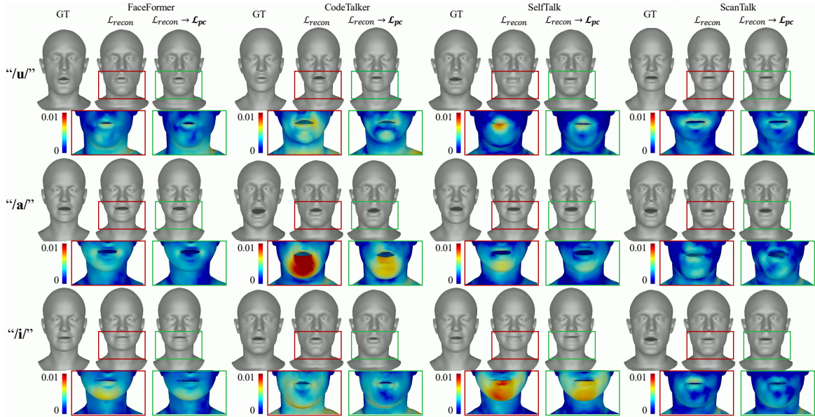
Figure 2: Visual comparisons of baseline models vs. baseline models trained with our objective function on VOCASET. Note that the second, fourth, and sixth rows represent the visualization of per-vertex errors in lip regions.
