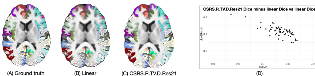
Figure 4: Panel (A) shows the original 1mm 3 resolution ground truth image and its segmentation. Panel (B) shows the impact of linear/generic label upsampling of ground truth data artificially downsampled to 2mm 3 . Panel (C) shows a CSRS result where other models are visually similar to this. Panel (D) demonstrates that all regions improve with CSRS (all differences > 0) and that regions with lower Dice overlap under the linear/generic label model improve more when upsampled with CSRS.
