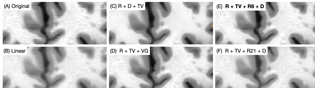
Figure 3: Comparison of CSRS with different loss functions to original resolution and linear upsampling. The bold (panel E) is the best performing model according to quantitative criteria. However, visual differences between the perceptual models (D,E,F) are not easy to discern.
