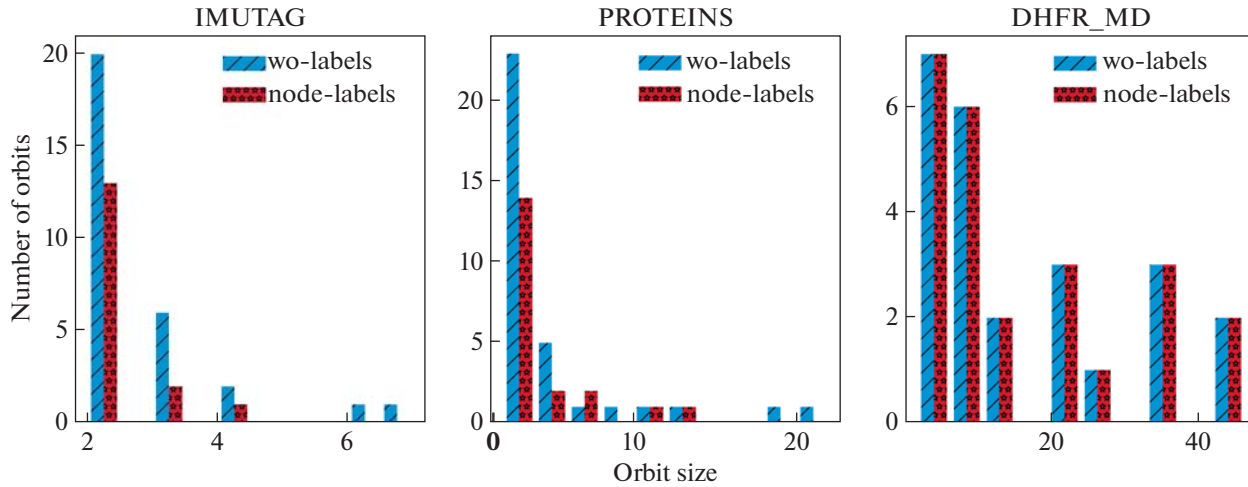
Fig. 2. Examples of distributions of orbit sizes with node labels.
