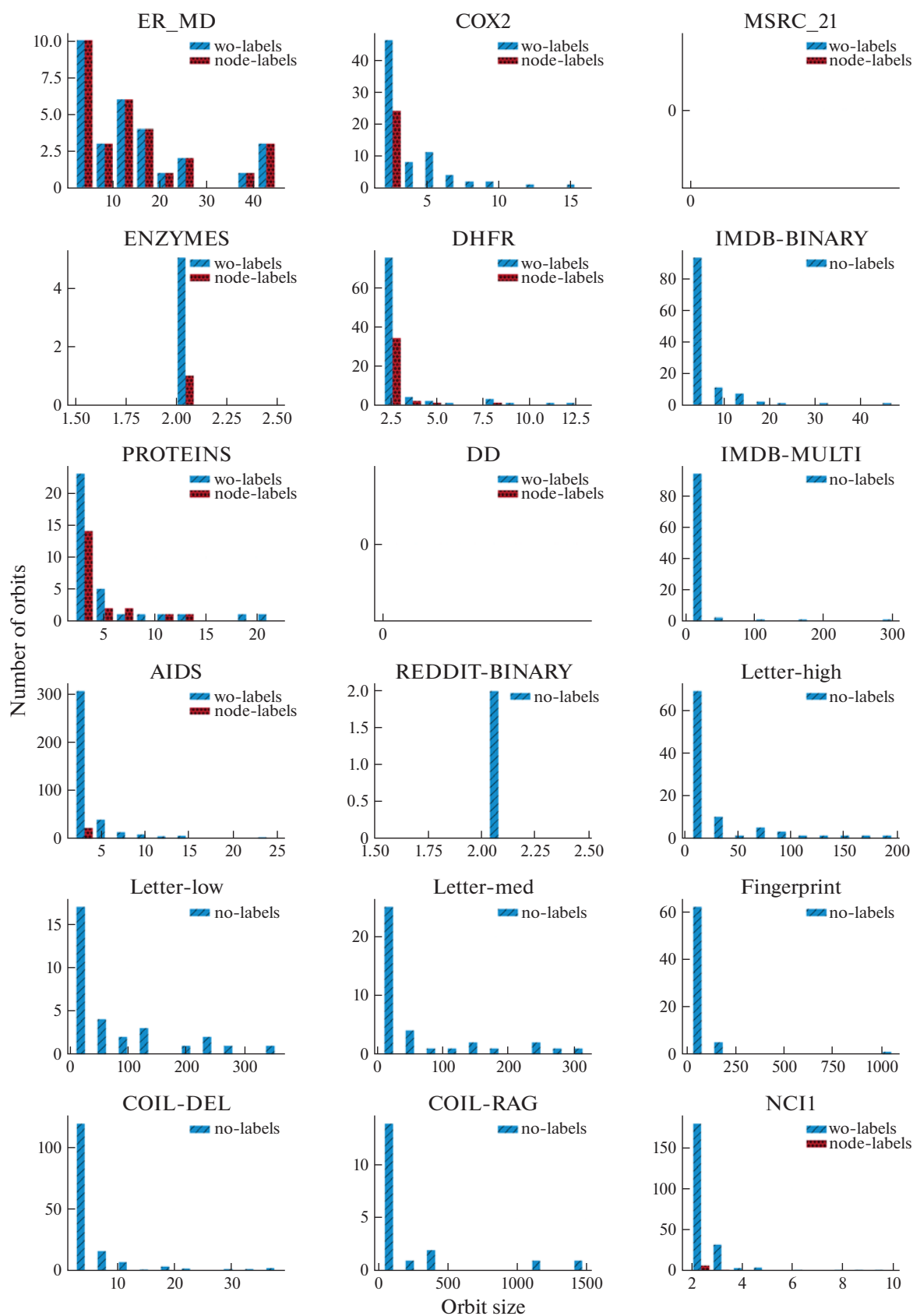
Fig. 4. Distribution of orbits sizes. Part-2.
