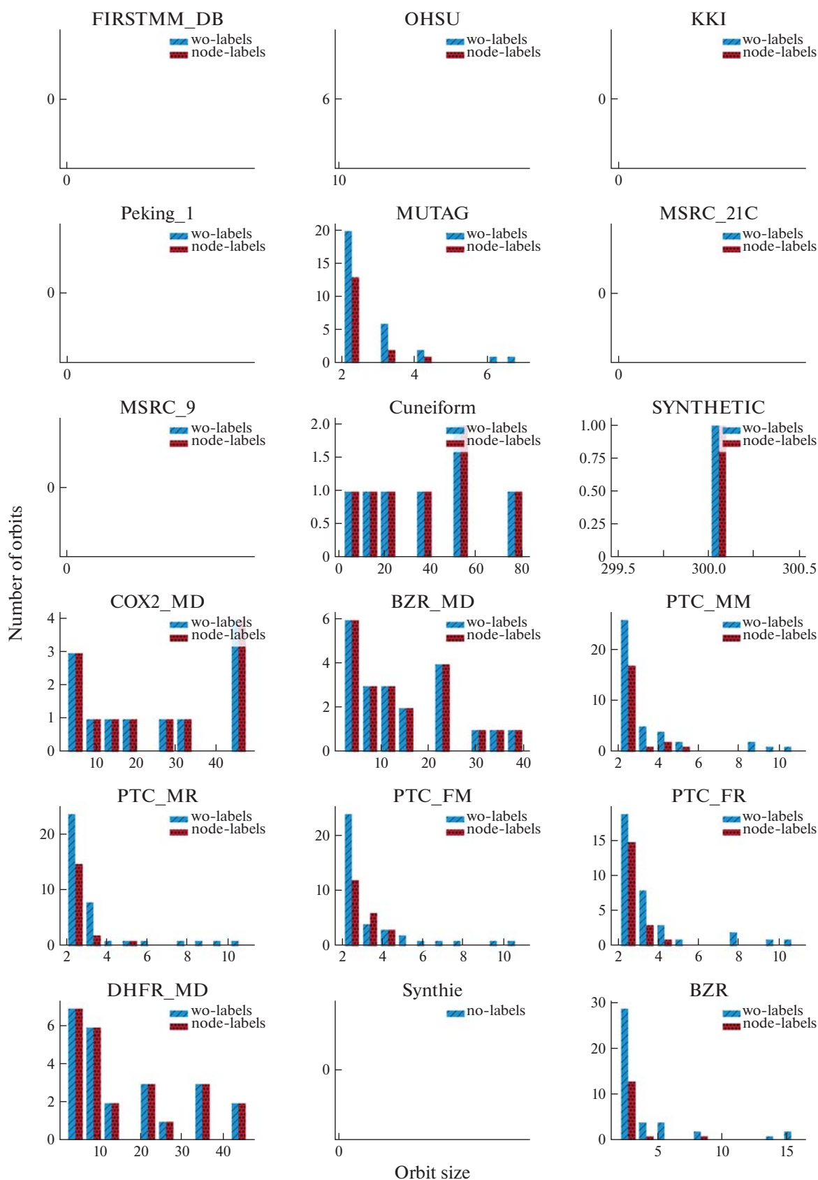
Fig. 3. Distribution of orbits sizes. wo-labels correspond to isomorphism without considering the labels. node-labels correspond to isomorphism that considers node labels. Part-1.
