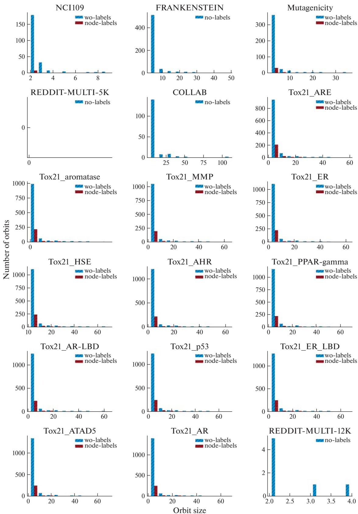
Fig. 5. Distribution of orbits sizes. Part-3.
