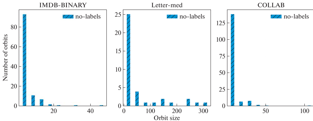
Fig. 1. Examples of distributions of orbit sizes without considering labels.
