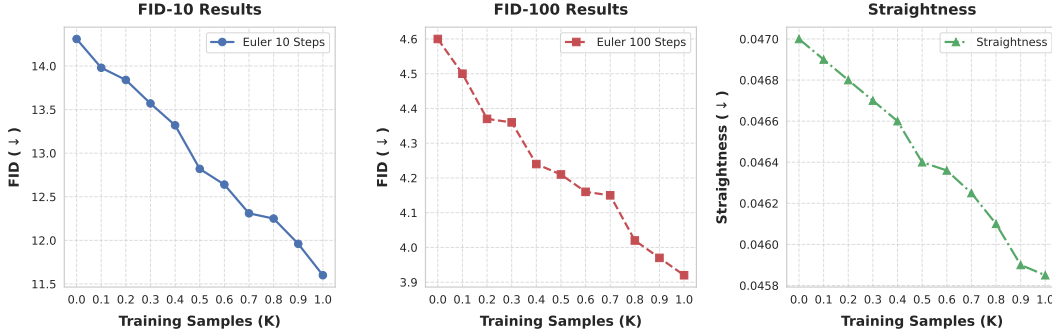
Figure 5 . Stability analysis of OAT-FM fine-tuning on CIFAR-10. Starting from a pre-trained FM model (400K batches), we refine the model using OAT-FM for an additional 1K training samples, recording metrics every 0.1K samples. We track generation quality (FID with 10 and 100 Euler steps) and flow straightness.
