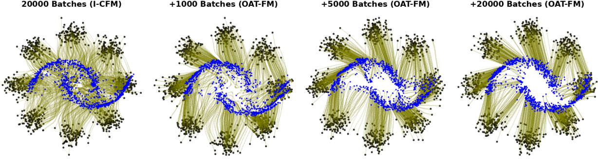
Figure 2 . An illustration of refining the flow of I-CFM via OAT-FM on the eight Gaussians to the Moons dataset. We conduct this experiment based on the code base provided in (Tong et al., 2024).
