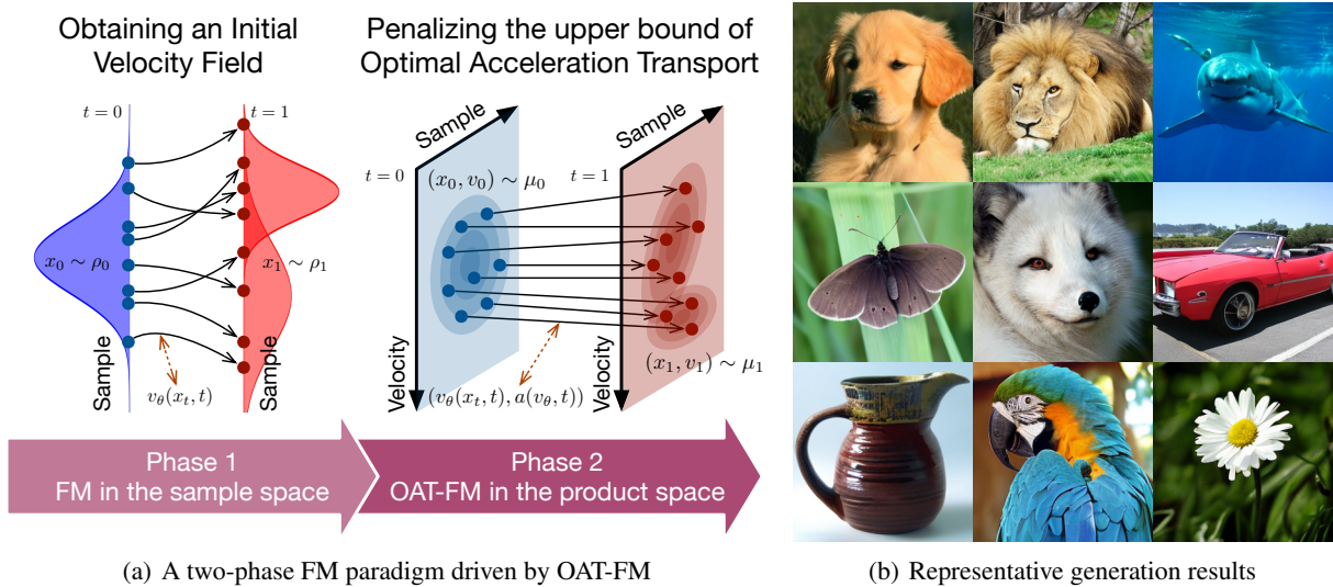
Figure 1 . (a) The principle of OAT-FM and the corresponding two-phase FM paradigm. (b) We train SiT-XL (Ma et al., 2024) by our two-phase FM paradigm on the ImageNet 256 \times 256 dataset (Deng et al., 2009).
