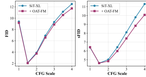
Figure 3 . The comparison of SiT-XL and SiT-XL + OAT-FM on FID and sFID.
