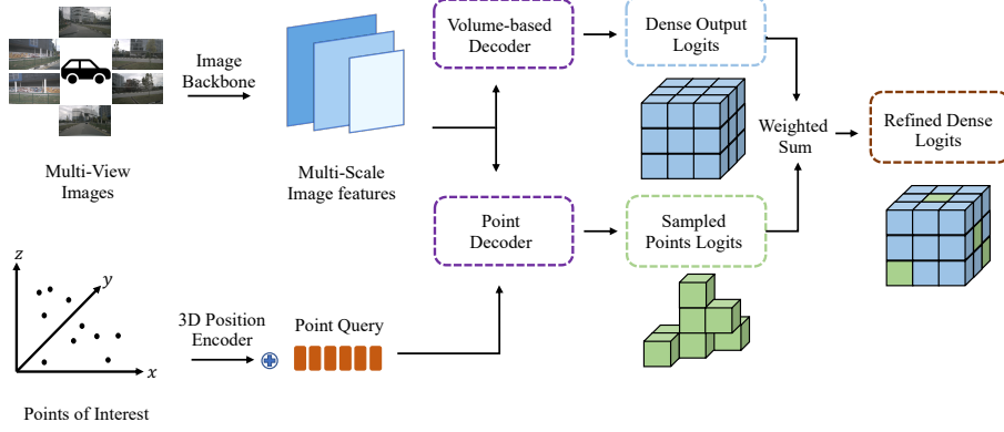
Fig. 3: Pipeline of refining volume-based methods with OSP. Given RGB images, 2D features are extracted by the frozen image backbone of the volume-based method which in our case is the BEVFormer baseline. We use the volume-based decoder to infer the entire scene, the point decoder to infer our selected 3D points, and combine the results of both using a weighted sum method.
