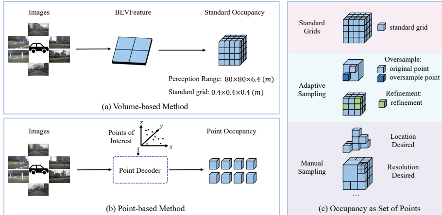
Fig. 1: Comparison between volume-based methods and our method. The volume-based methods, represented by BEVFormer, infer every region within the scene and get standard occupancy as shown in (a). Our method uses a point-based decoder as shown in (b). Thus it infers the Points of Interest including standard, adaptively sampled, and manually sampled grids as shown in (c).
