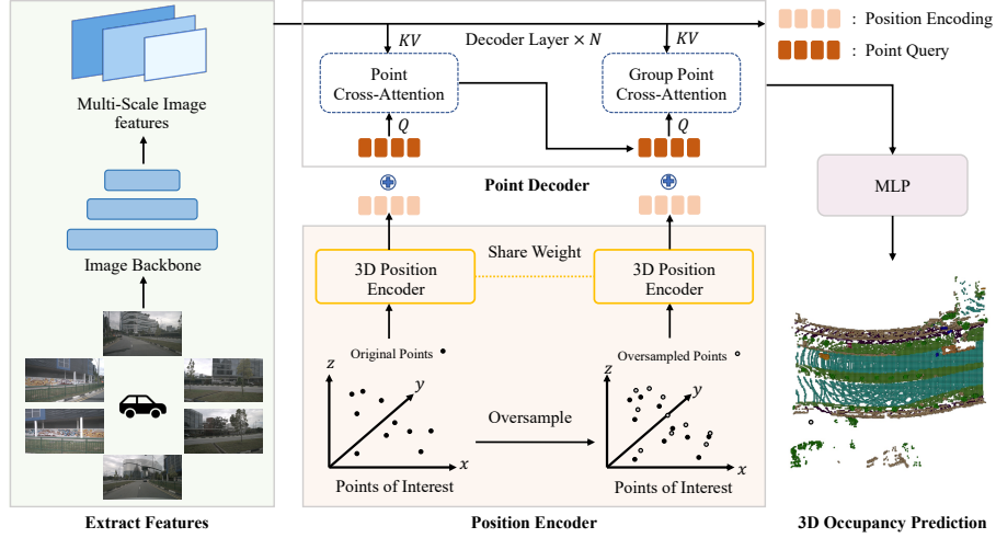
Fig. 2: Overall framework of Occupancy as Set of Points. OSP leverages the Transformer architecture to derive 3D point features from 2D images to make 3D occupancy predictions. Initially, we extract 2D features from multi-view images. Following this, we employ a set of 3D point queries to index these 2D features. The selection of these 3D point queries depends on the Points of Interest (PoIs).
