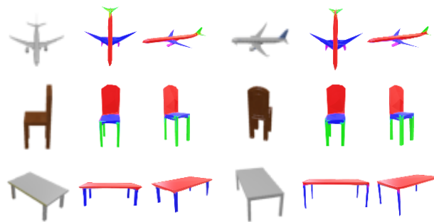
Figure 1. This paper aims at learning partonomic 3D reconstruction from an image collection with only 2D annotations. Our goal is not only to reconstruct the shape of an object from a single-view image but also to decompose the shape into meaningful semantic parts. The first and fourth columns are single-view input images. The other columns are partonomic 3D reconstruction results obtained by our proposed approach.
