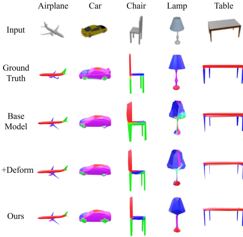
Figure 6. Qualitative ablation study on ShapeNetPart. The base model uses the CST representation and predicts a global latent vector for partonomic reconstruction. +Deform means to extend the base model with the PDF representation but predict object and part latent vectors through MLPs.
