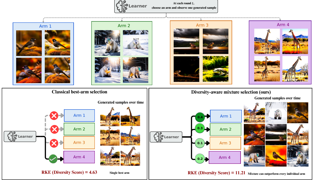
Figure 1: Classical multi-armed bandits seek the best single arm with the highest expected reward. However, for diversity-aware objectives, the score can be strictly higher for a non-degenerate mixture of the arms. For example, in the generative model bandit setting, the optimal mixture solution is usually an interior point of the probability simplex, assigning non-zero probability to multiple generators (arms). We demonstrate that this geometric property can naturally encourage exploration and study whether explicit UCB exploration is necessary in diversity-aware multi-armed bandit settings.
