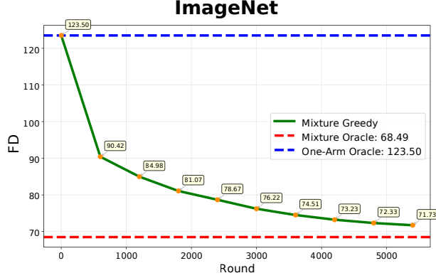
Figure 5: Convergence of FD in ImageNet dataset generative models.
