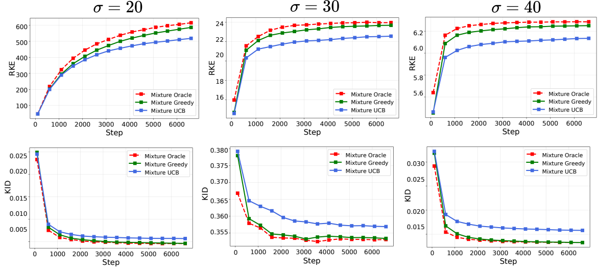
Figure 11: Convergence of KD and RKE for generative models trained on FFHQ dataset using three bandwidths
