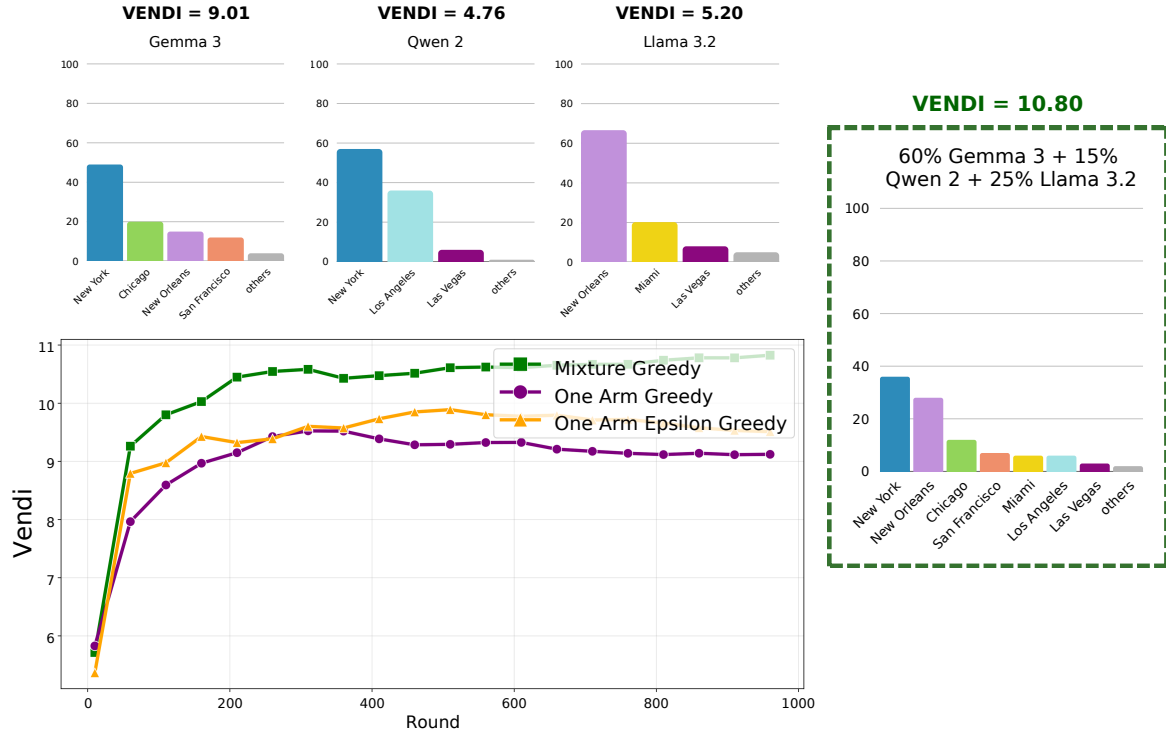
Figure 9: Application of Mixture Greedy on LLM generated texts to optimize Vendi Score.
