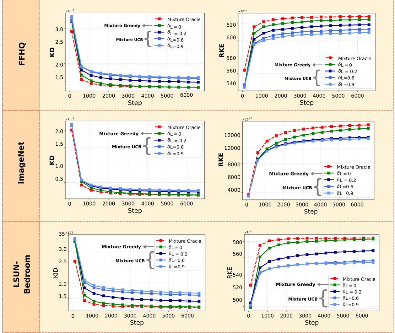
Figure 7: Comparison of KD and RKE convergence among different datasets.
