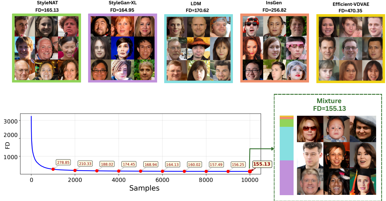
Figure 4: Mixture Greedy, minimizing Frechet Distance using exponentiated gradient descent on FFHQ generated samples.
