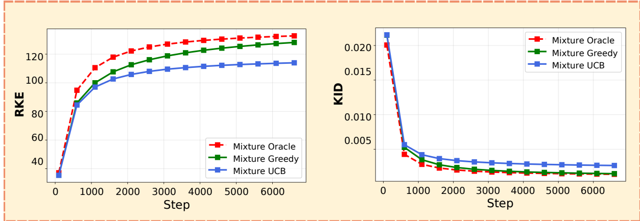
Figure 2: Comparison of mixture selection strategies over five ImageNet pretrained generative models from Stein et al. [2023]’s repository in terms of RKE \uparrow (left) and KID \downarrow (right) of generated samples from step 1 to t (plots’ x-axis). Mixture-Greedy performed better than Mixture-UCB [Rezaei et al., 2025] (with the UCB exploration term) in both the experiments with RKE and KID objectives. Mixture-Oracle always generates samples from the population-optimal mixture of models.
