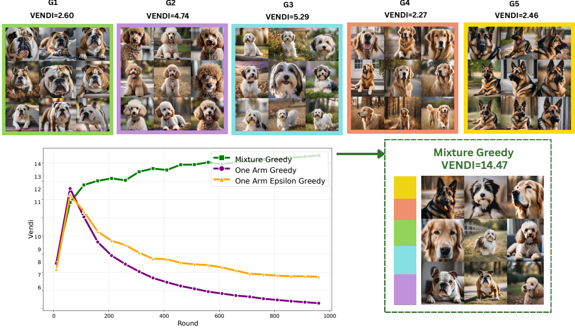
Figure 8: Application of Mixture Greedy on generated dog breeds dataset to optimize Vendi Score.
