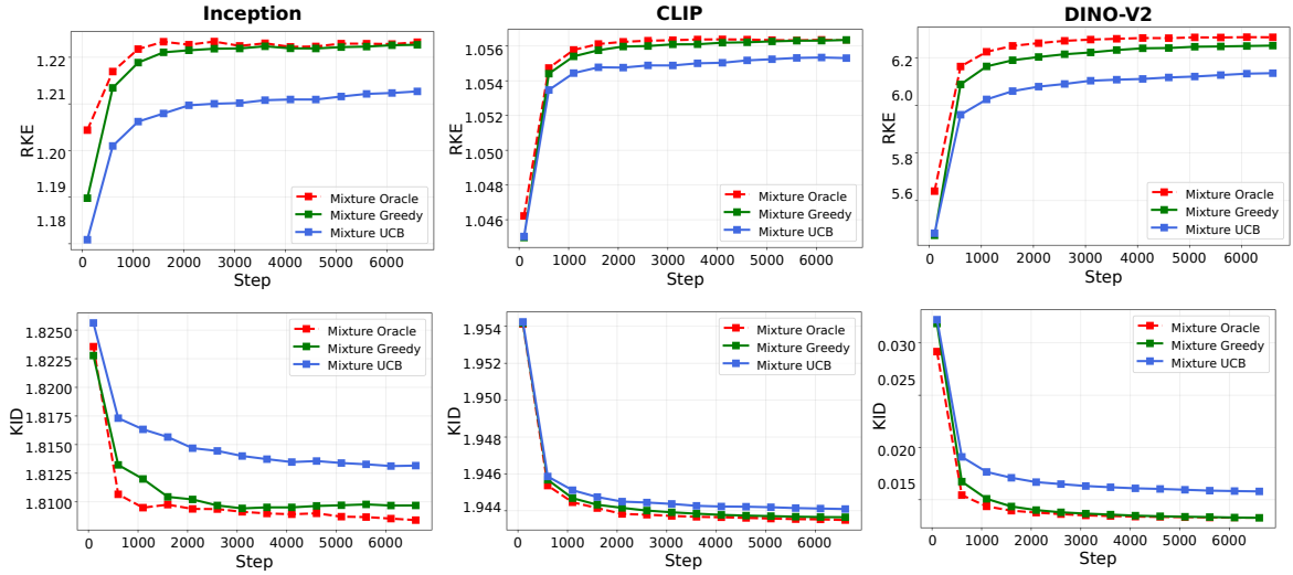
Figure 12: Convergence of RKE and KD on FFHQ generative models, using different feature extractors.
