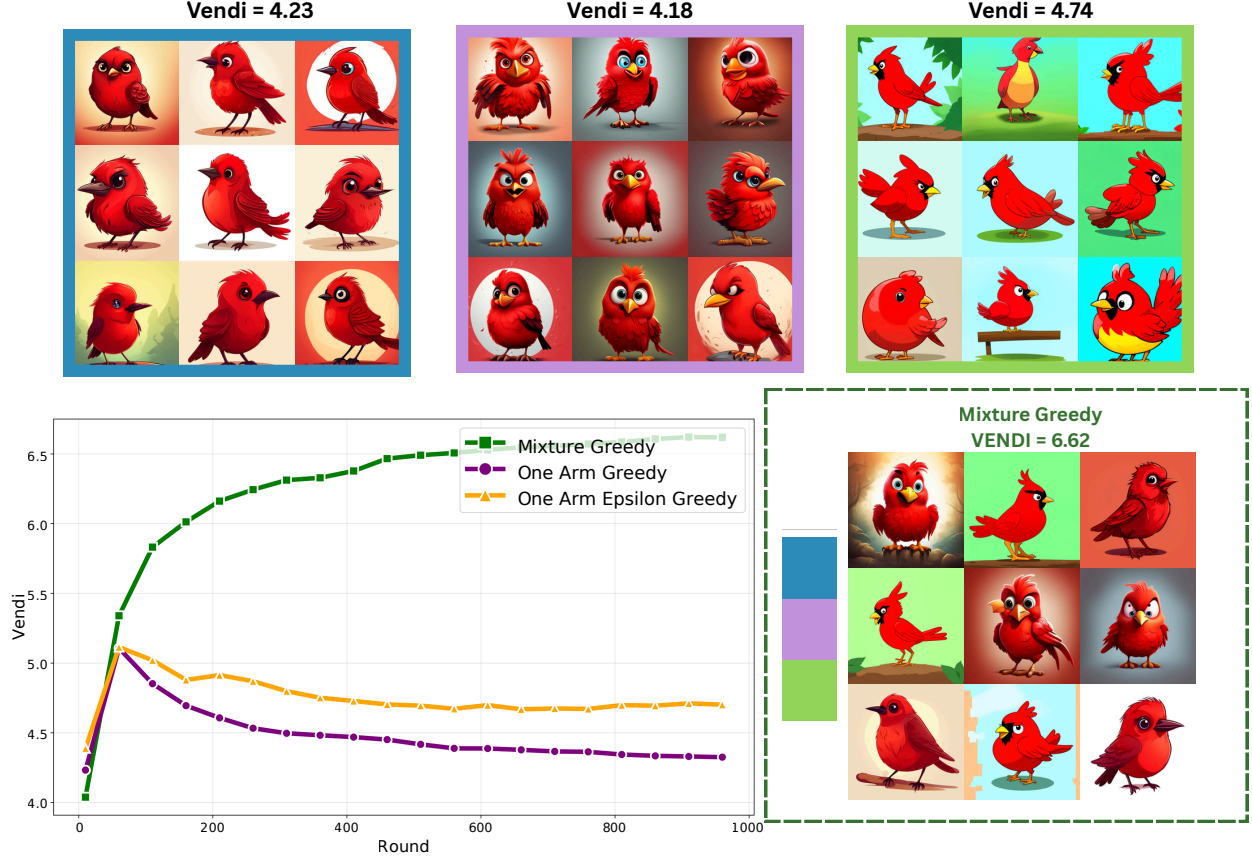
Figure 6: Application of Mixture Greedy on the generated red birds dataset to optimize Vendi Score.
