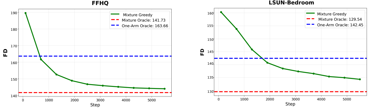
Figure 3: Convergence of Mixture Greedy to the Mixture Oracle in terms of Fréchet Distance (FD) across image selection steps on FFHQ (left) and LSUN-Bedroom (right).
