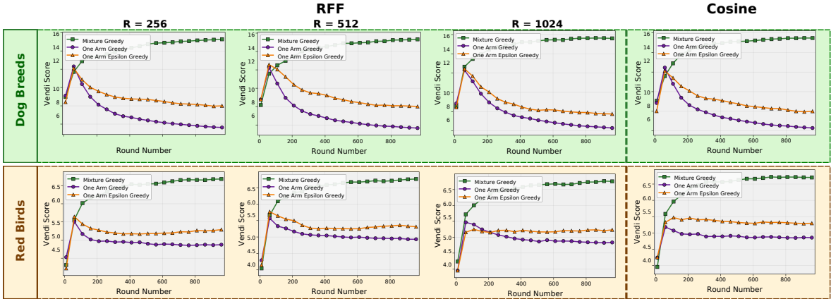
Figure 10: Vendi score over rounds for different using RFF (R=256/512/1024) and cosine kernel on two generated datasets.
