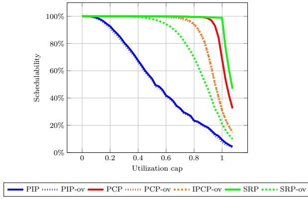
Fig. 6: Selected results for single-processor setup (periods heterogeneous, long critical sections).
