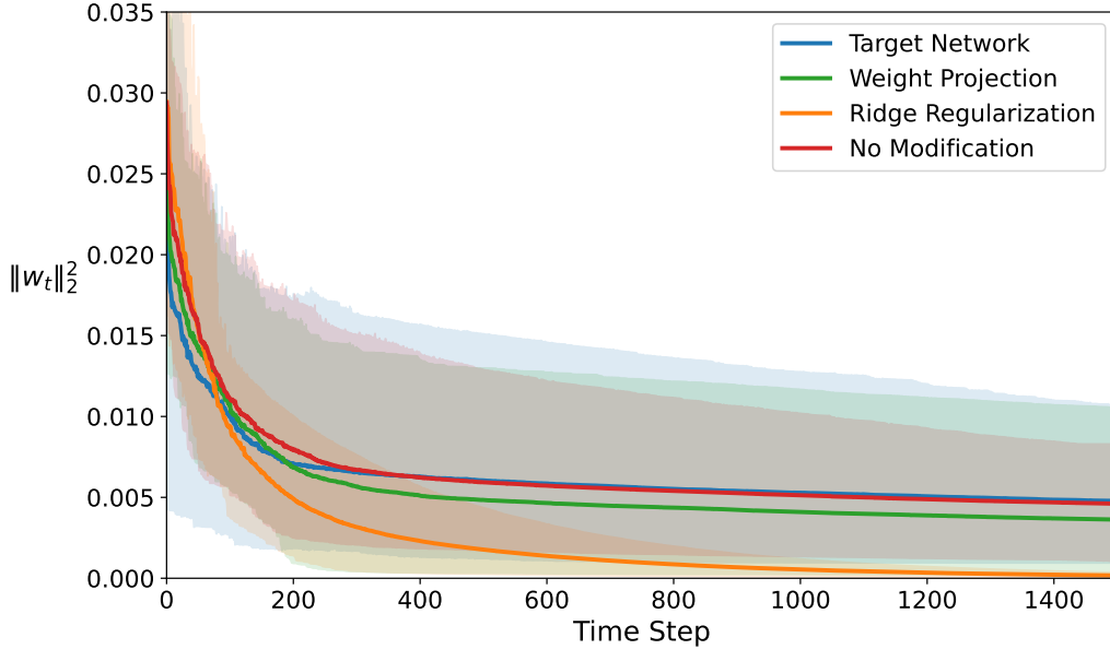
Figure 2. Each scenario is independently run 10 times, with the solid lines representing the averages of the squared L^2 norm of weights, and the shaded areas indicating the ranges between minimum and maximum values. This comparison illustrates the impact of different modification strategies on the algorithm’s convergence behavior.
