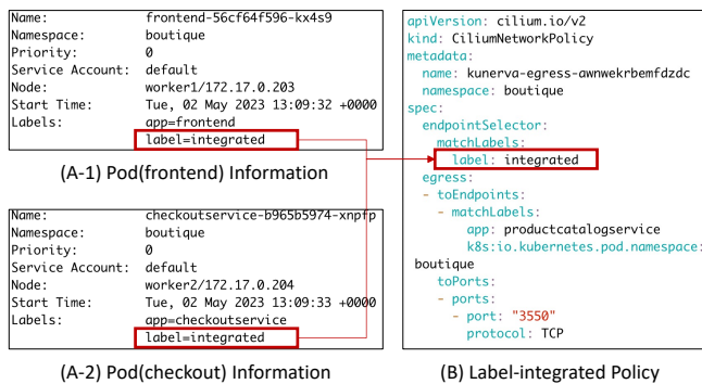
FIGURE 14: The regenerated network policy specification resulting from label integration.
