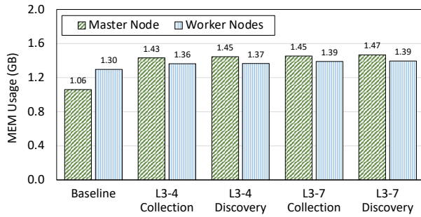
FIGURE 18: Measurements of the changes in MEM usage with different combinations of KUNERVA components.
