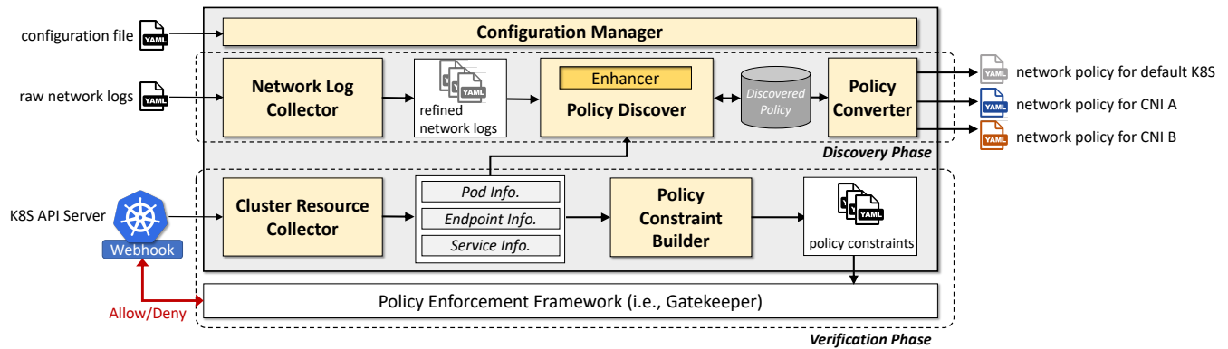
FIGURE 3: Overall architecture of KUNERVA with six key components; (i) Configuration Manager, (ii) Network Log Collector, (iii) Policy Discover, (iv) Policy Converter, (v) Cluster Resource Collector, and (vi) Policy Constraint Builder.
