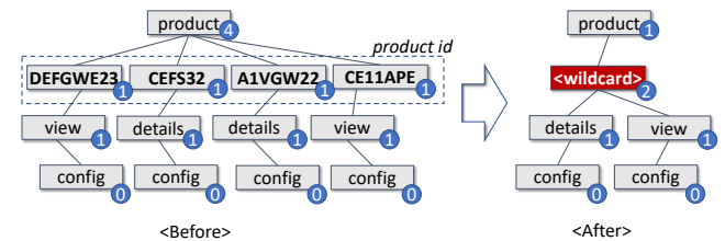
FIGURE 8: An example of an L7 dependency tree. The number within each circle refers to the count of child nodes.
