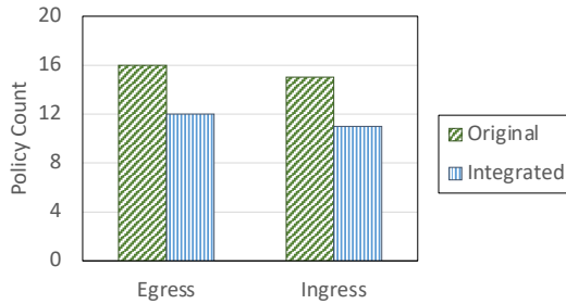
FIGURE 13: Measurements of the changes in the number of policies resulting from label integration.
