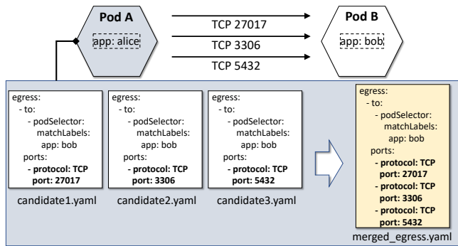
FIGURE 6: An example of merging multiple policy candidates into a single network policy.
