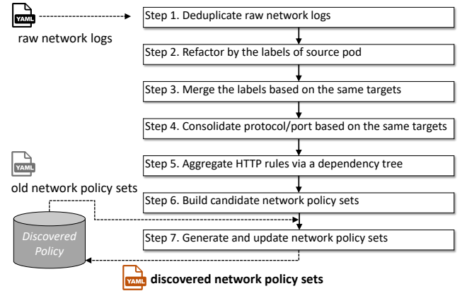
FIGURE 4: Workflow for discovering a network policy.
