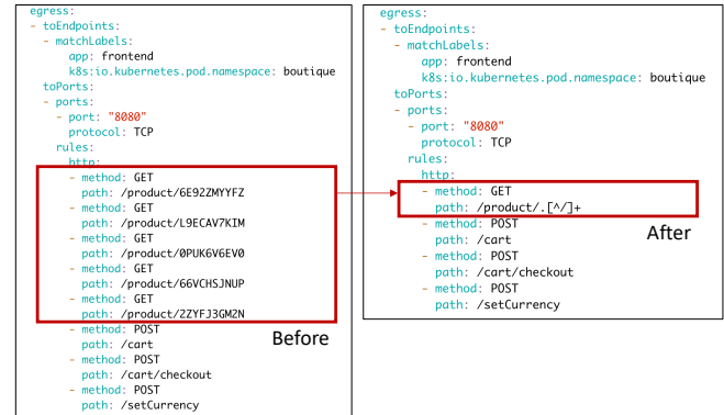
FIGURE 15: Results of toHTTP rule aggregation.
