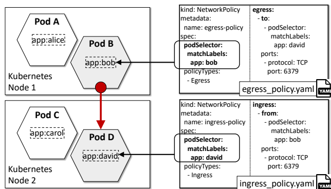
FIGURE 2: Example of network policy enforcement in cluster. Dashed-line box refers to the label assigned to each pod.
