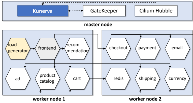
FIGURE 12: Test environments and deployed microservices. The solid lines represent traffic between the pods, while dashed ones indicate traffic that our framework interacts with.
