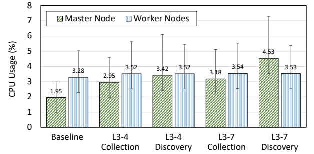
FIGURE 17: Measurements of the changes in CPU usage with different combinations of KUNERVA components.
