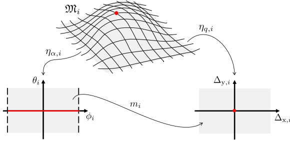
Fig. 1. The chart \eta_{\alpha,i} classically used to describe the configuration manifold \mathcal{M}_i of a continuum soft segment with constant curvature generates artificial redundancies and singularities, which in turn produce pathological behaviors when controlling the robot. These characteristics are artificial in the sense that they are not a physical property of the system, but instead they are introduced by its mathematical description. In this work we analyze a set of coordinates \Delta_{x,i}, \Delta_{y,i} alternative to the classic \phi_i, \theta_i . They are identified by a chart \eta_{q,i} which we prove defining an atlas, i.e. it maps the whole \mathcal{M}_i one-to-one in the Euclidean space - solving the discussed issues. This reflects in strongly improved performance in simulating and controlling the robot.
