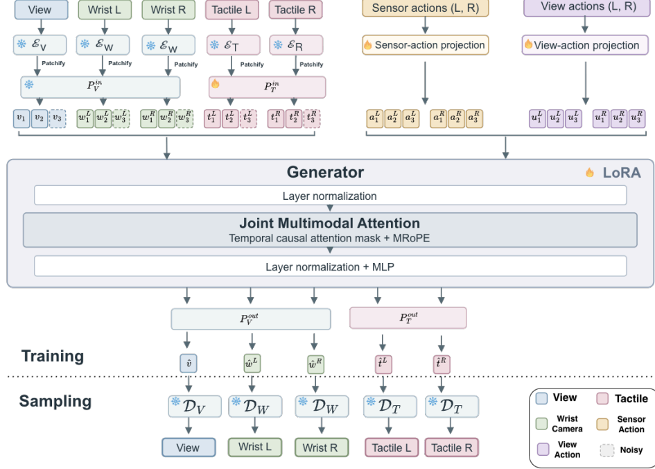
Figure 2: Overview of ACTS. Frozen encoders produce observation latents, whose spatial patches are mapped to tokens by input projectors P^{in} . A generator initialized from pretrained Cosmos3 weights jointly processes noisy future tokens conditioned on clean history, force-aware sensor actions, and view-aligned actions. Output projectors P^{out} map target-token features to latent velocity predictions. The scene and two wrist streams share the RGB projector pair (P_V^{in}, P_V^{out}) , while both tactile streams share (P_T^{in}, P_T^{out}) . Sampling updates only future latents, which frozen decoders reconstruct into synchronized multimodal predictions.
