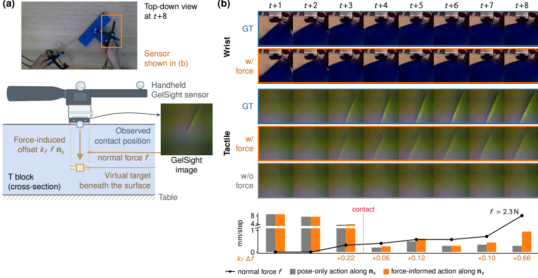
Figure 1: Force-informed sensor actions. (a) Top: scene view, with the sensor of (b) boxed. Estimated normal force f shifts the sensor target by k_f f \mathbf{n}_s along the gel normal, so each action includes k_f \Delta f \mathbf{n}_s (Eq. 3). (b) On a held-out PushT sequence, the force-conditioned model forms the tactile imprint at contact, while the pose-only model does not. Tactile crops are shown at 2\times contrast.
