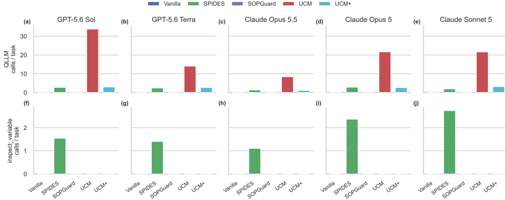
Figure 7: Mean security-mechanism tool calls per valid utility-task run across models and defenses. QLLM counts calls to the quarantined model; inspect_variable counts explicit reveals into the main model’s context.
