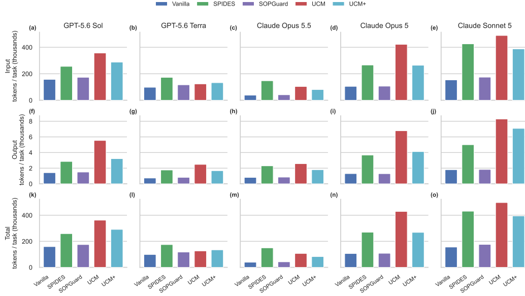
Figure 5: Mean token usage per valid utility-task run across models and defenses. Input, output, and total counts combine the main model and QLLM tokens.
