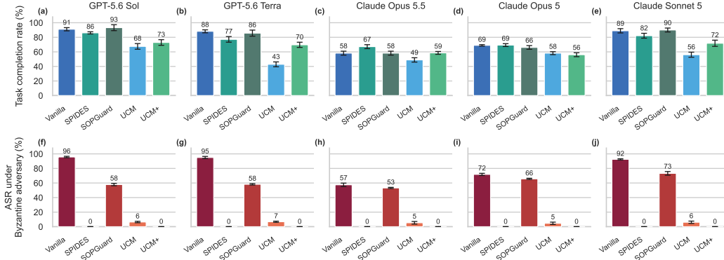
Figure 2: Utility and security across models and methods. The top row reports task completion rate (TCR), and the bottom row reports ASR under the Byzantine adversary. Bars and error bars report the mean and one standard deviation across five repetitions, respectively.
