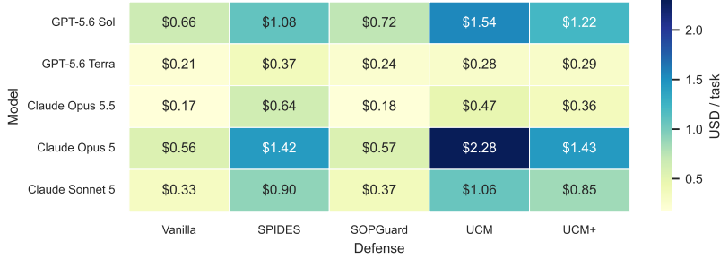
Figure 6: Estimated mean token cost in USD per valid utility-task run. Estimates use GitHub Copilot’s default-tier token prices as of September 25, 2026.
