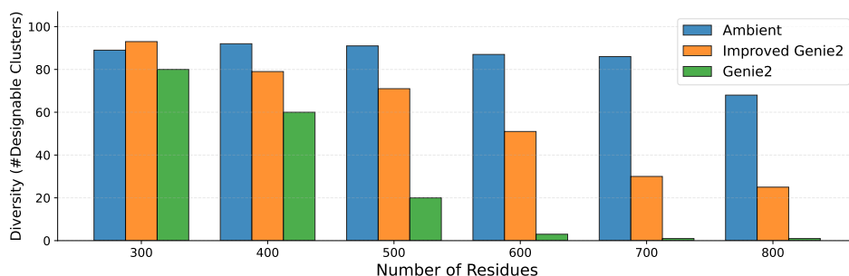
Figure 4: Ablation to quantify the effect of the Ambient Protein Diffusion framework. We improve upon Genie2 by making the architecture bigger, reclustering the dataset as in Section 3.3 and by finetuning on longer proteins (up to 768 aminoacids). The resulting improved Genie2, shown in Orange, outperforms Genie2 but still lags behind our Ambient Protein Diffusion Model, shown in blue. The only difference between the two models is that Ambient Protein Diffusion uses low pLDDT AlphaFold structures as noisy data, as explained in Section 3.2. Ambient Protein Diffusion consistently outperforms both the improved Genie2 baseline and Genie2, with increasingly significant improvements as sequence length grows.
