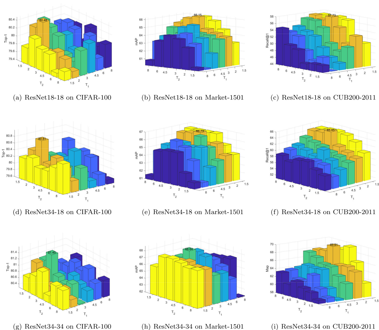
Fig. 3 Results on CIFAR-100, the mAP accuracy (%) on Market-1501, and the Recall@1 accuracy (%) on CUB200-2011 with varying temperatures T_1 and T_2 using ResNet18-18, ResNet34-18 and ResNet34-34 as the teacher-student architectures
