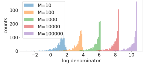
Figure 1: Histogram of \log \sum_{i=1}^M p(\tilde{\mathbf{z}}_2^{(i,n)} | \bar{\mu}_2^{(j)}) with respect to different M \in \{10^1, 10^2, 10^3, 10^4, 10^5\} . Distributions shift by roughly a constant when M increases by 10 times, implying the denominator scales proportionally to M .
