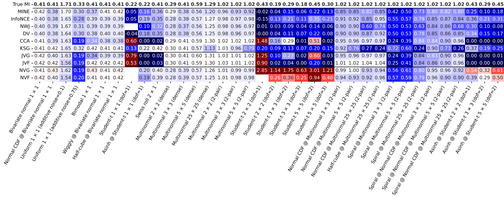
Figure 5: MI Benchmark runs against a selection of 36 different scenarios. Blue indicates an underestimate and red indicates on overestimate with the magnitude indicated by saturation. Blank cells indicate that the method produced divergent estimates.
