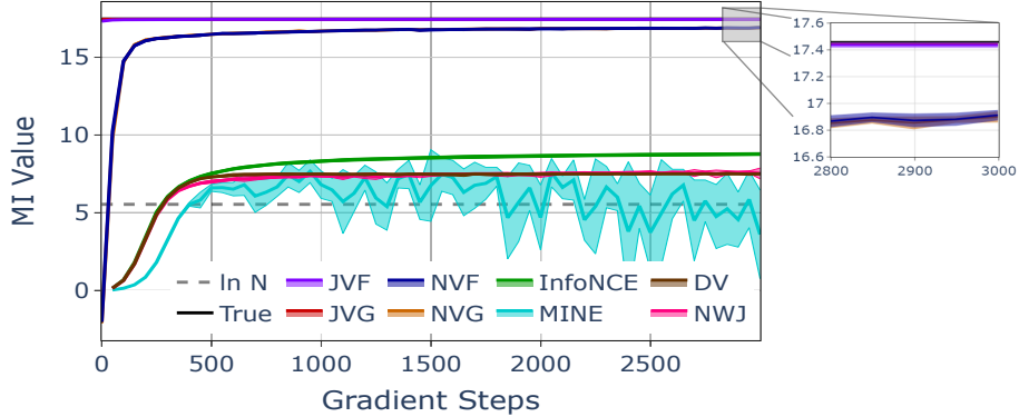
Figure 2: Large MI is difficult for many estimators to approximate. We see that the four distribution based estimators, I_{JVG} , I_{NVG} , I_{JVF} , and I_{NVF} , can accurately predict MI, but the four discriminative-based methods, MINE, InfoNCE, NWJ, and DV, all converge around \mathcal{O}(\log(N)) .
